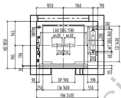
Hoistway plan/1:60
