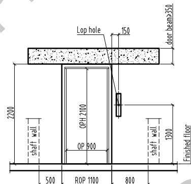
E/reserved hole/1: 60
