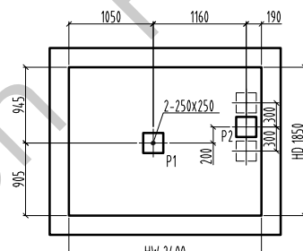
Pit plan/1: 60
