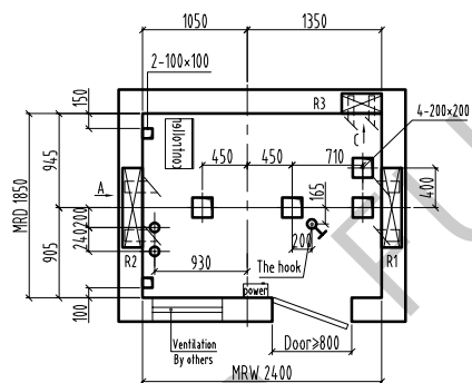
Machine room plan/1:60
