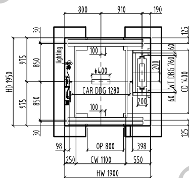
Hoistway plan/1:60
