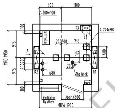
Machine room plan/1:60
