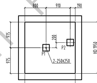
Pit plan/1:60
