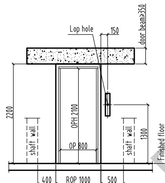
E reserved hole/1:60
