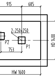
Pit plan/1:60
