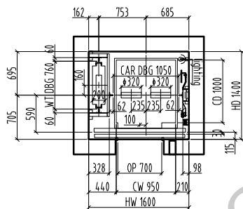
Hoistway plan/1:60
