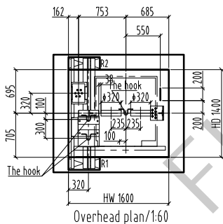
Overhead plan/1:60
